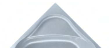
KAIRO (Left or right-handed, left-handed shown) Length (nominal): 1550mm Width (nominal): 950mm Tub depth (deepest point): 450mm
